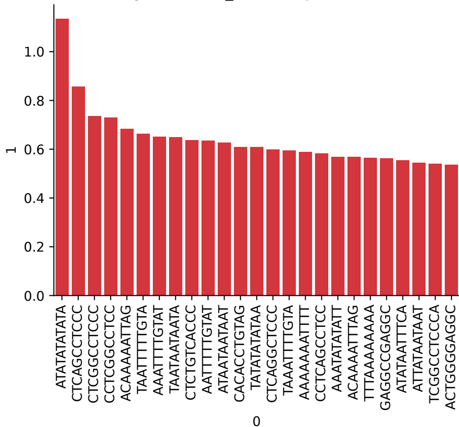
Isgkm SKNSH_95033 Top 25 kmers
